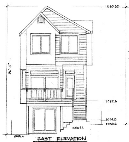
EAST ELEVATION
